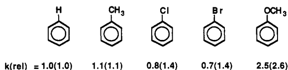
Figure 9. Relative reactivity of substituted benzenes toward nucleogenic vinyl cation. The data refer to competition experiments carried out at room temperature in liquid arenes. The data in parentheses refer to gas-phase competition experiments at room temperature.
