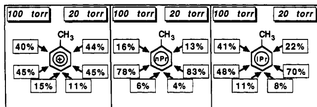
Figure 10. Isomeric distribution of tolylium ions, n -propyltoluenes, and isopropyltoluenes at 100 and 20 Torr of propane.
